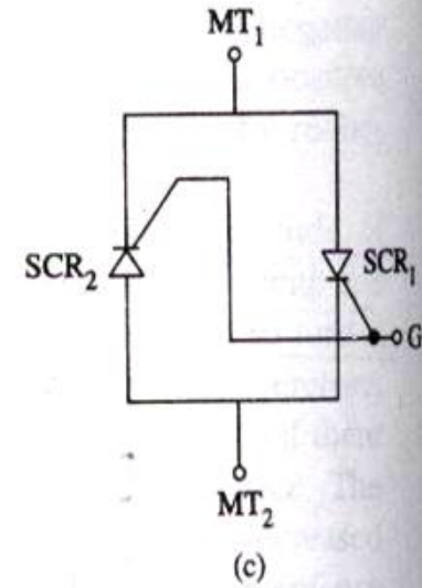
SCR equivalent circuit
